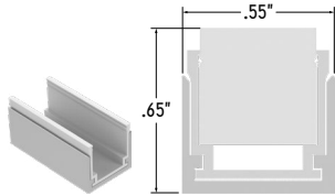
Mounting Clip (LLED9150-F-MC)
