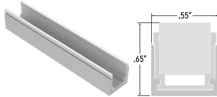
Mounting Channel (LLED9150-F-UC)
